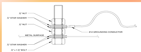
Example of Grounding Lug
